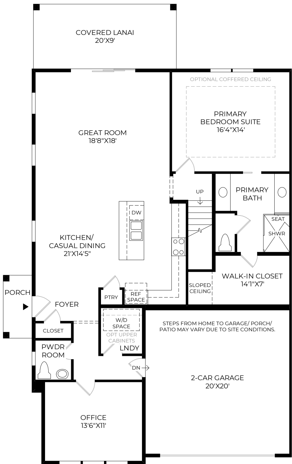
First Floor 10' CEILING HEIGHT
