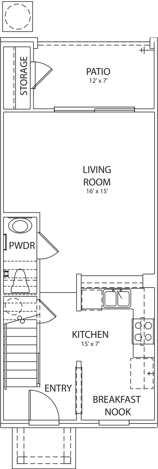
FIRST FLOOR
