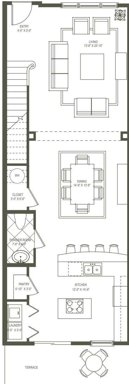
FIRST FLOOR MAY ST.
